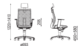
EXAMPLE OF INTRATA WITH HEIGHT ADJUSTABLE ARMRESTS
