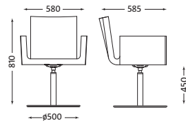
VICTORIA 1S weight: 25,6 kg
