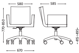
VICTORIA ST33 weight: 14,5 kg
