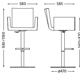
VICTORIA HOCKER weight: 26,8 kg
